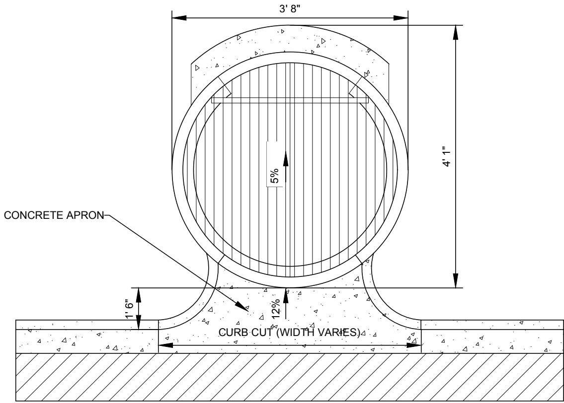
PLAN VIEW
